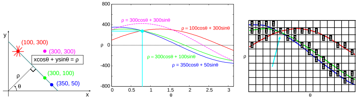
図 6: Hough 変換.
